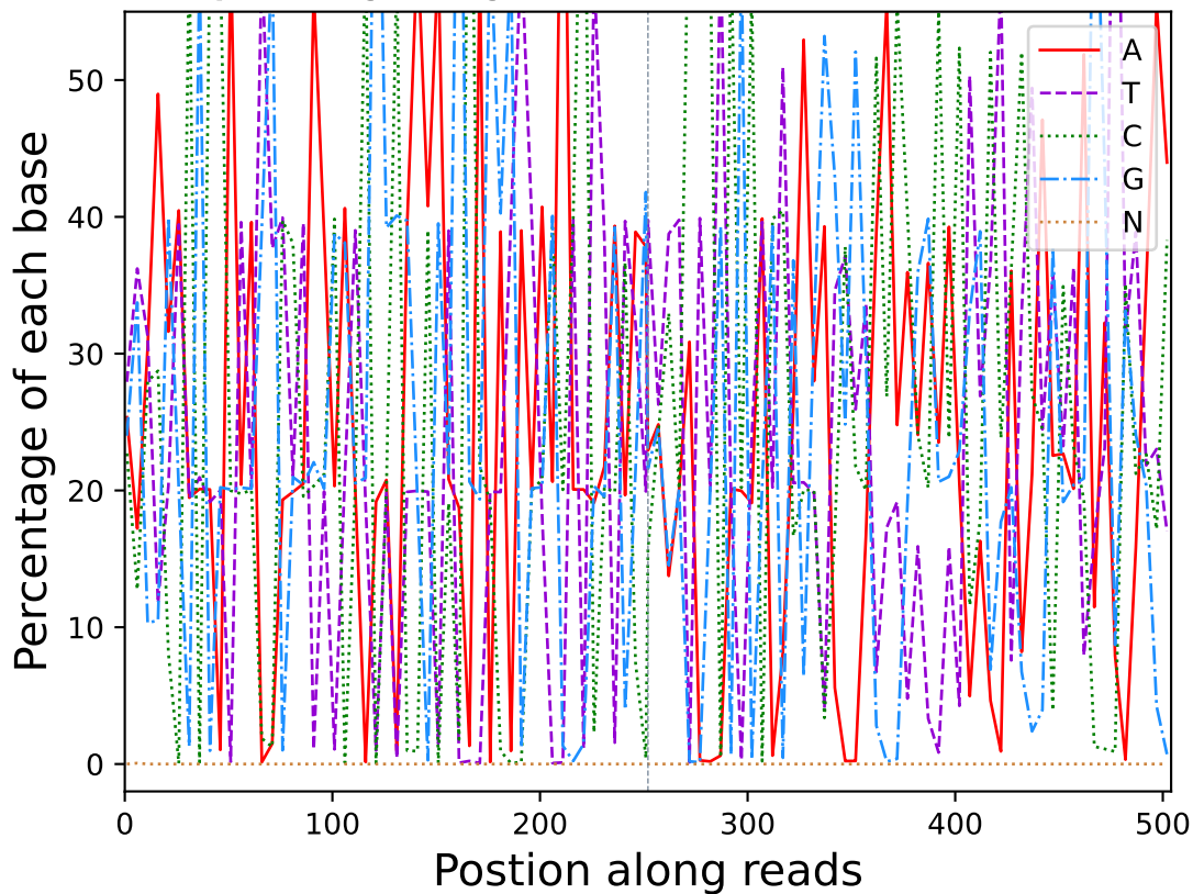
Base percentage along reads (R20212)
